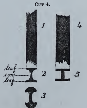
Diagram, shewing the width and profile of ancient and modern leads.
